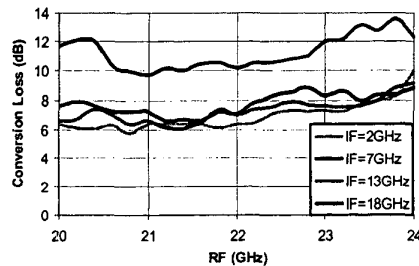
Fig. 14. Measured conversion loss across RF band
