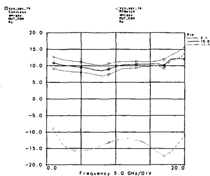
Fig. 10. Final simulated performance of the upconverter
