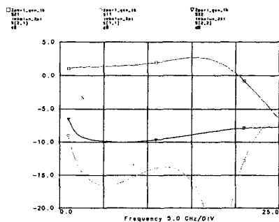
Fig. 9. Two-port simulation of the active balun
