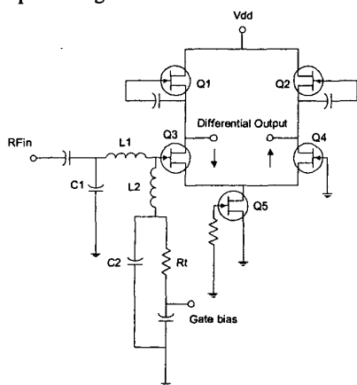
Fig. 8. Input stage of IF active balun
