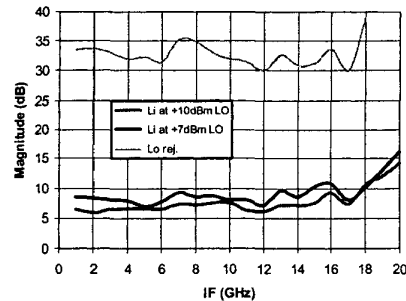
Fig. 13. Measured conversion loss and LO rejection of the upconverter IC
