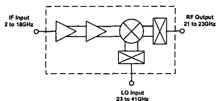
Fig. 2. MMIC architecture
